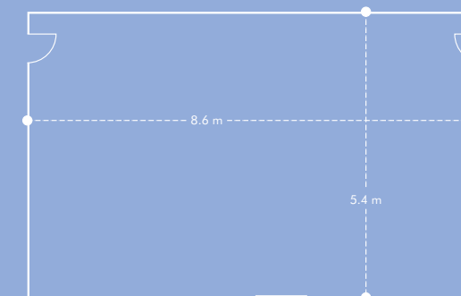
Floor plan for Surf View PATIO DOORS
